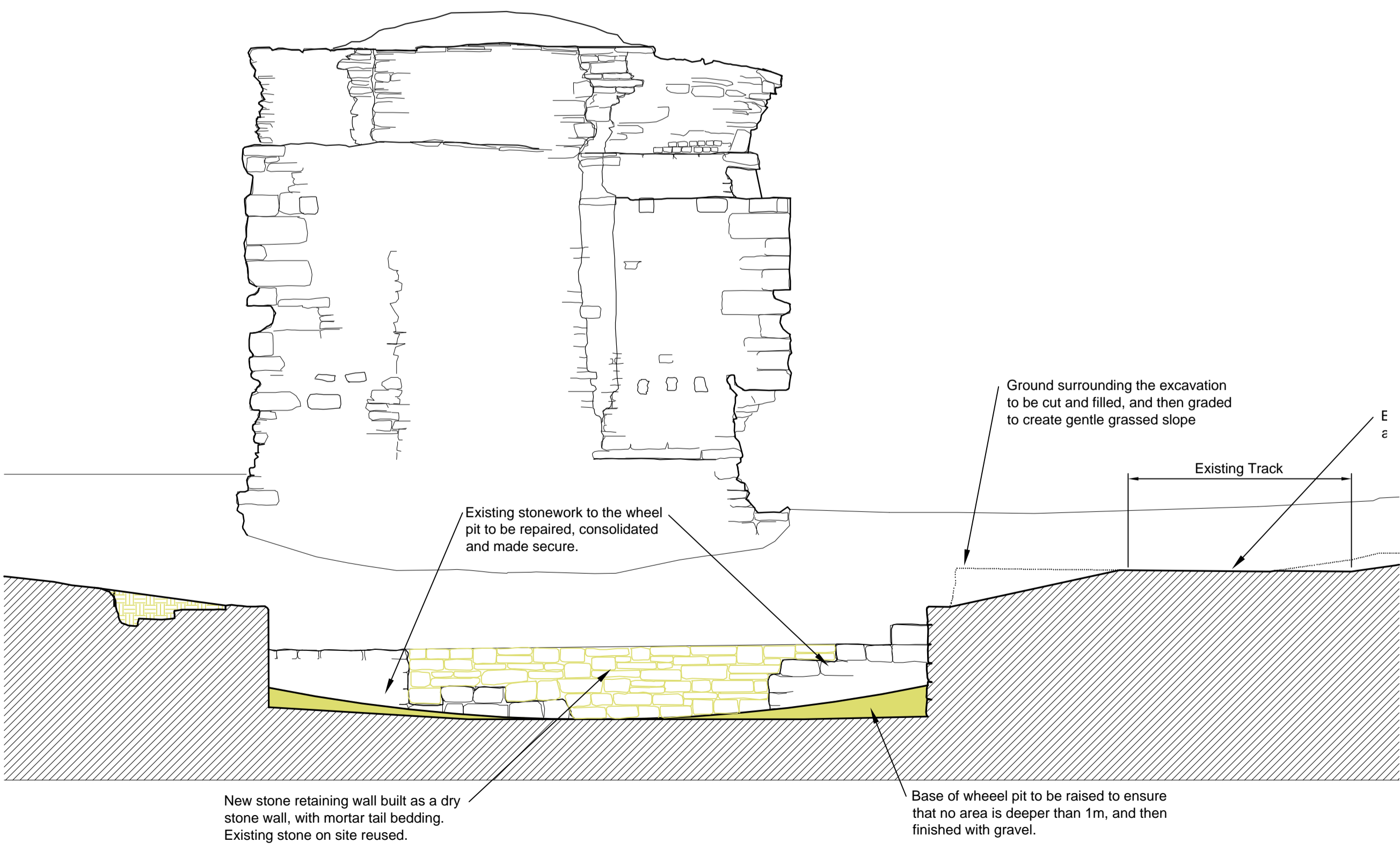
PROPOSED EAST WEST SECTION 1:50
