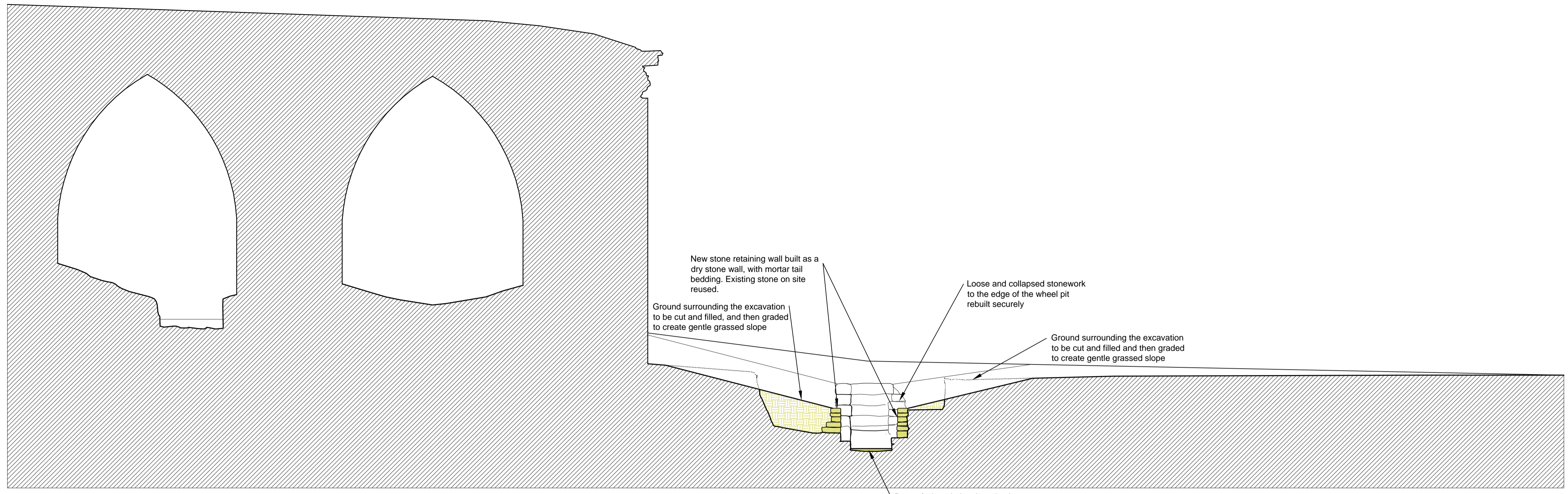
PROPOSED NORTH SOUTH SECTION 1:50
