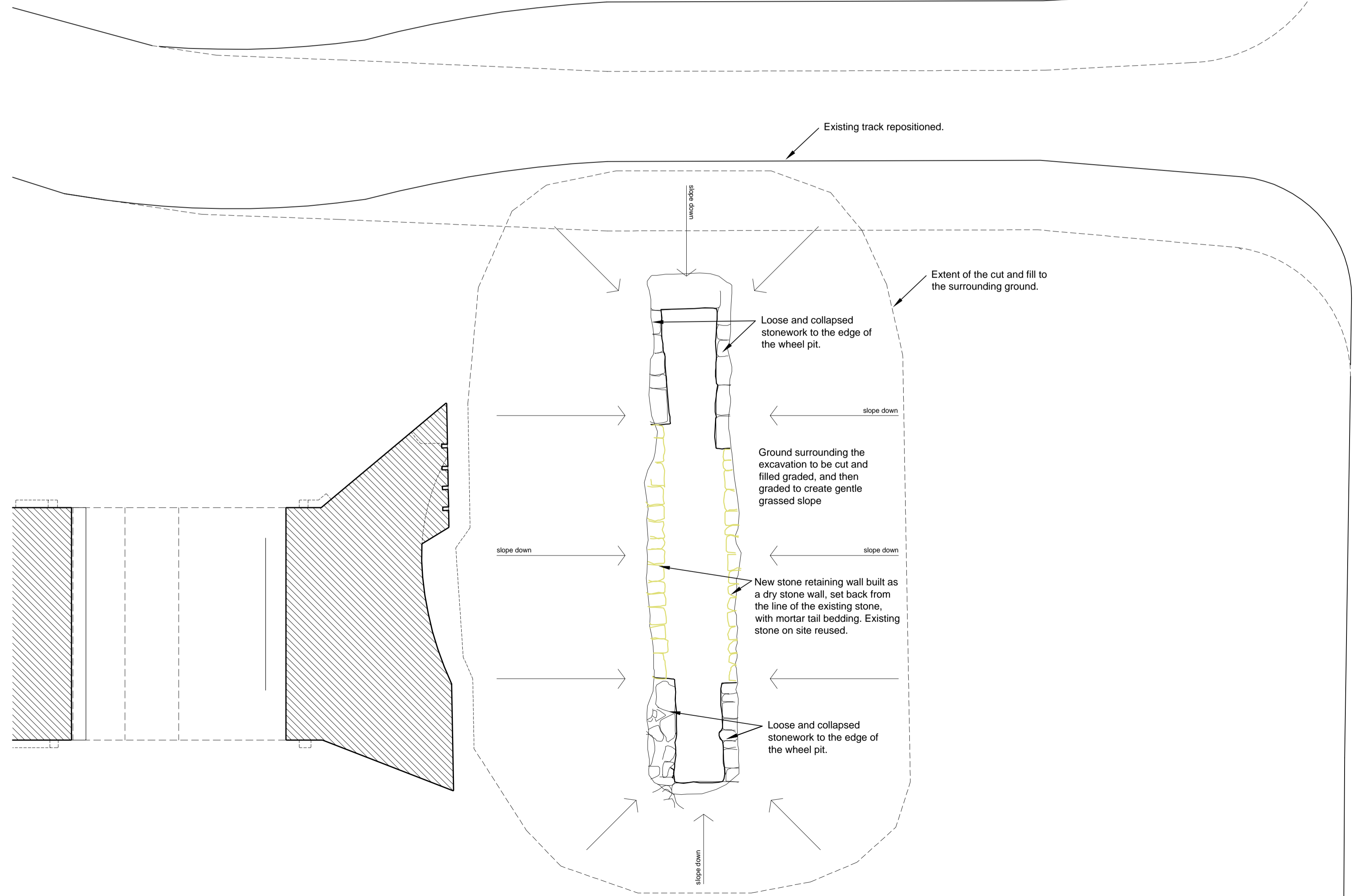
PROPOSED PLAN OF EXCAVATED WHEEL PIT 1:50
