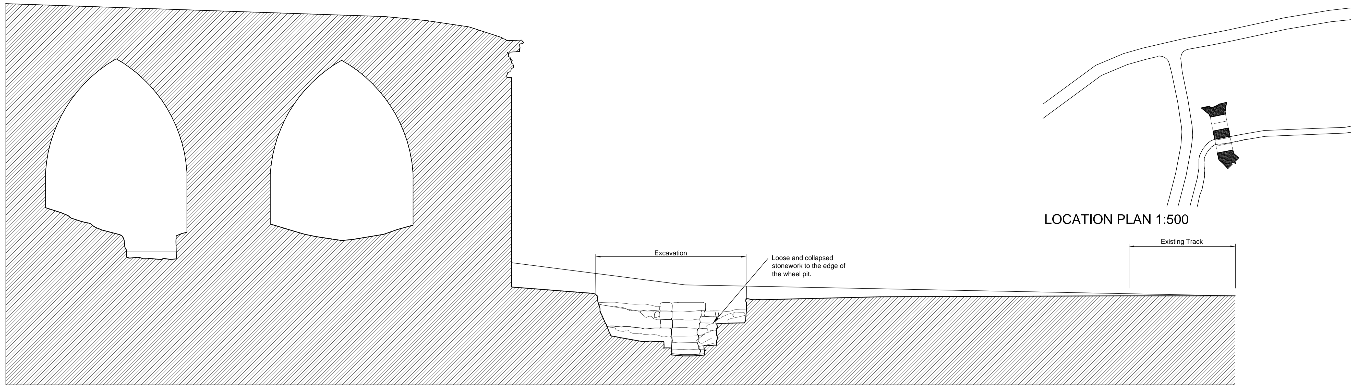
EXISTING NORTH SOUTH SECTION 1:50
